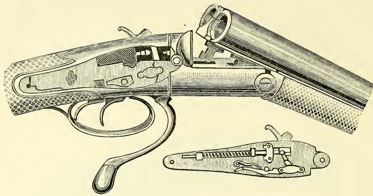
Langs' Self-cocking Gun, with Dummy Hammers.
